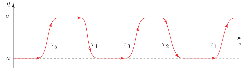
Figure 3.8: Dilute instanton gas configuration.
