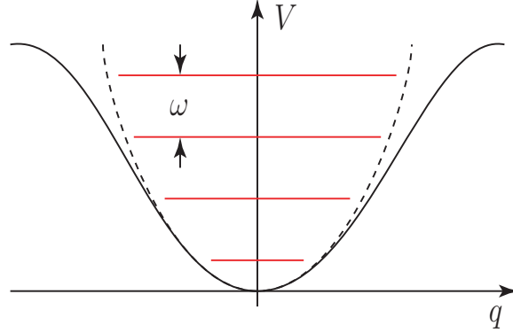
Figure 3.5: Solid: Potential well. Dashed: Quadratic fit approximating the potential shape close to the minimum.
